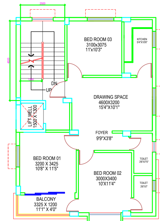
FLOOR PLAN: 3BHK LAYOUT
