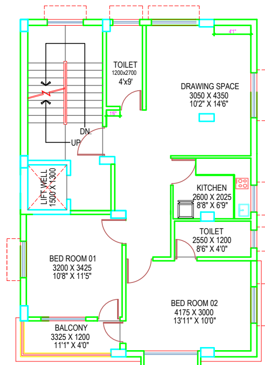
FLOOR PLAN: 2BHK LAYOUT
